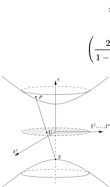
Fig. 3.5: Hyperbolic stereographic projection
